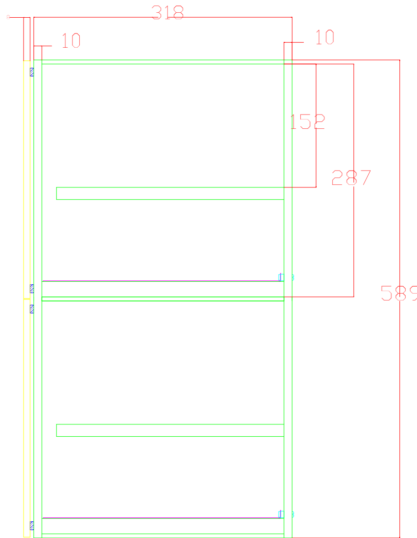
3100-02 Side Elevation
