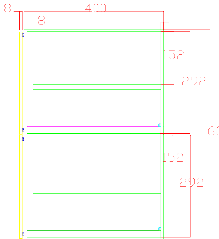
3100-03 Side elevation
